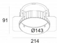
MOUNTING KIT R143 TRIMLESS 202 15 61 97
